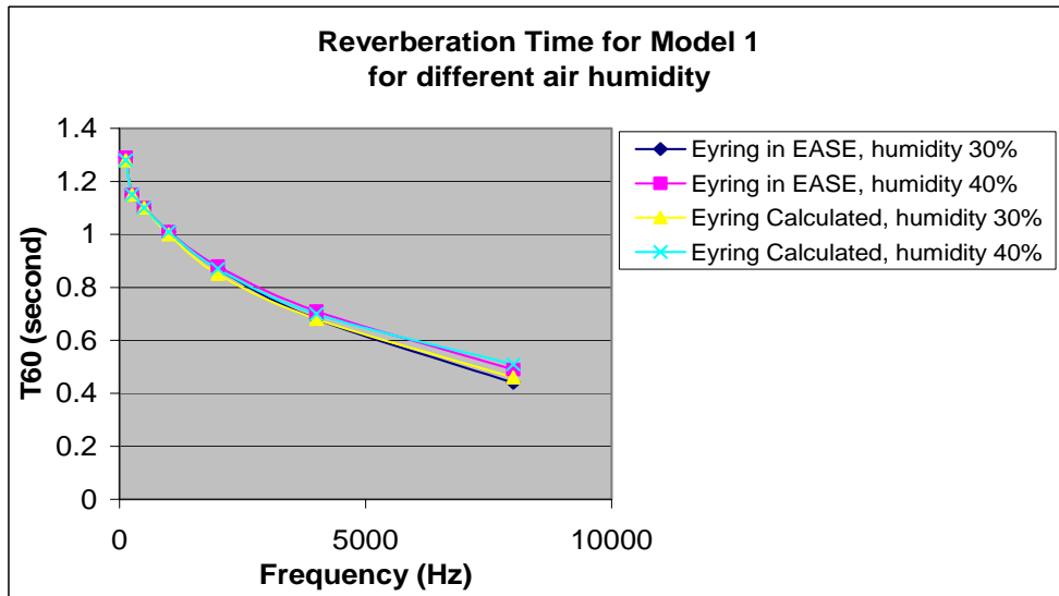
Figure 4.15. Chart of reverberation time in model 1, comparing values for 30% and 40% air humidity using results from EASE™ and numerical calculations.
